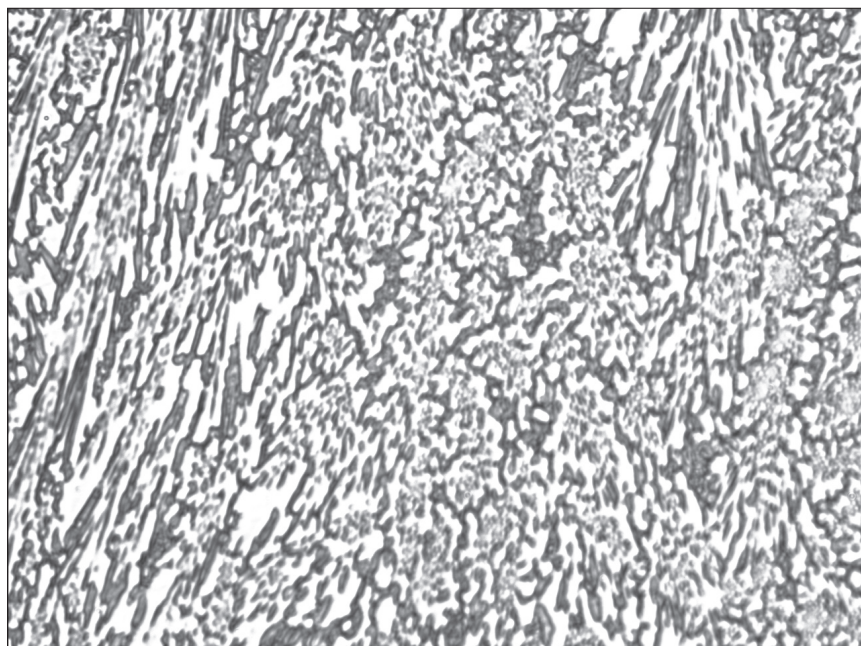
Optical micrograph of a Stellite® 1 weld overlay
